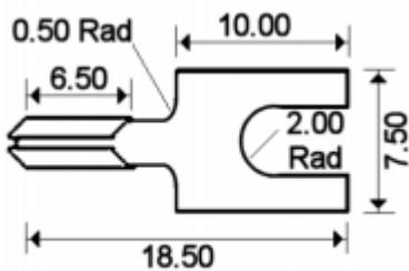
Thermocouple Spade Terminal
